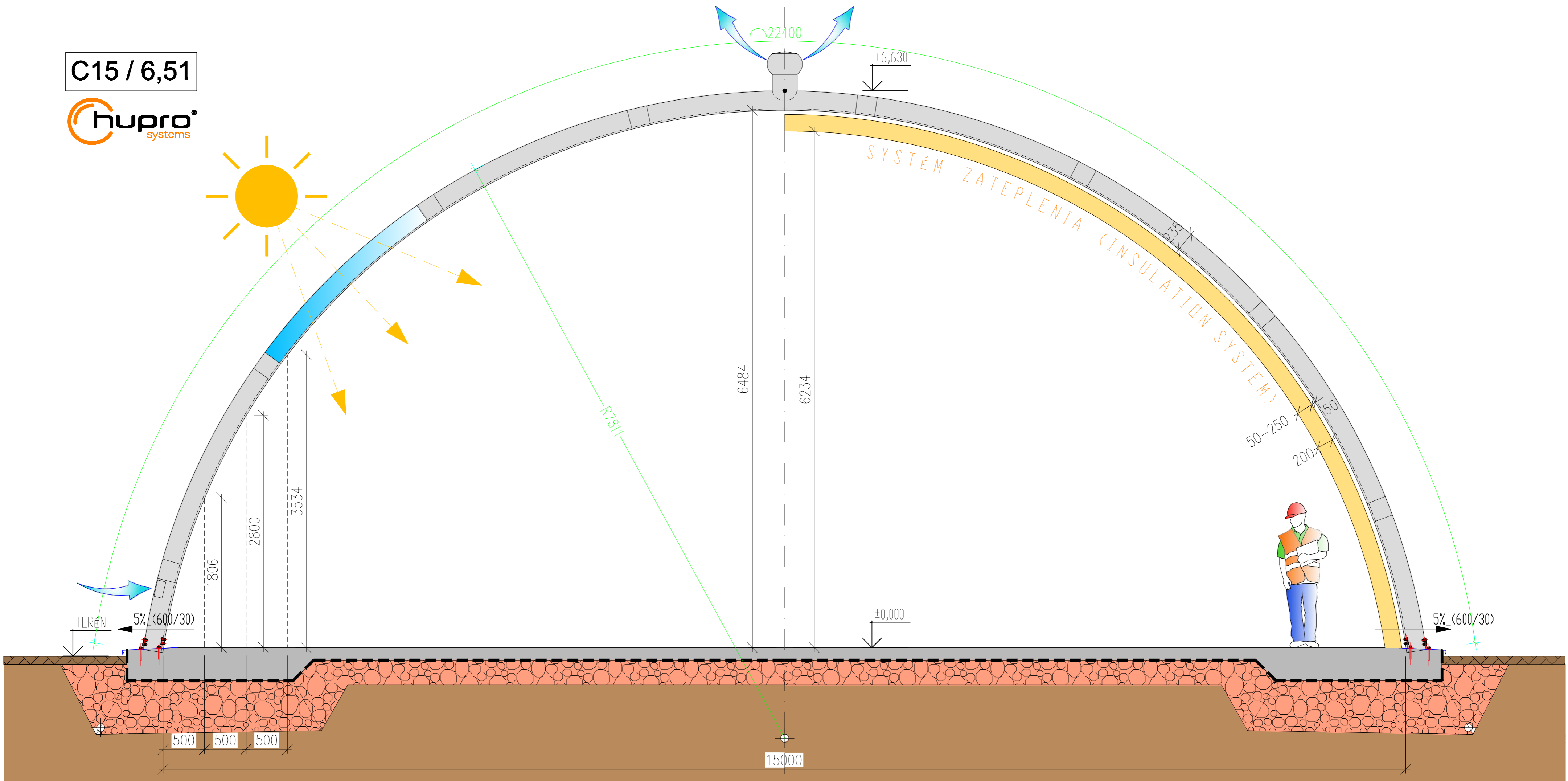
ORIENTAČNÝ TVAR ZAKLADANIA (ORIENTATION FORM OF FOUNDING)
