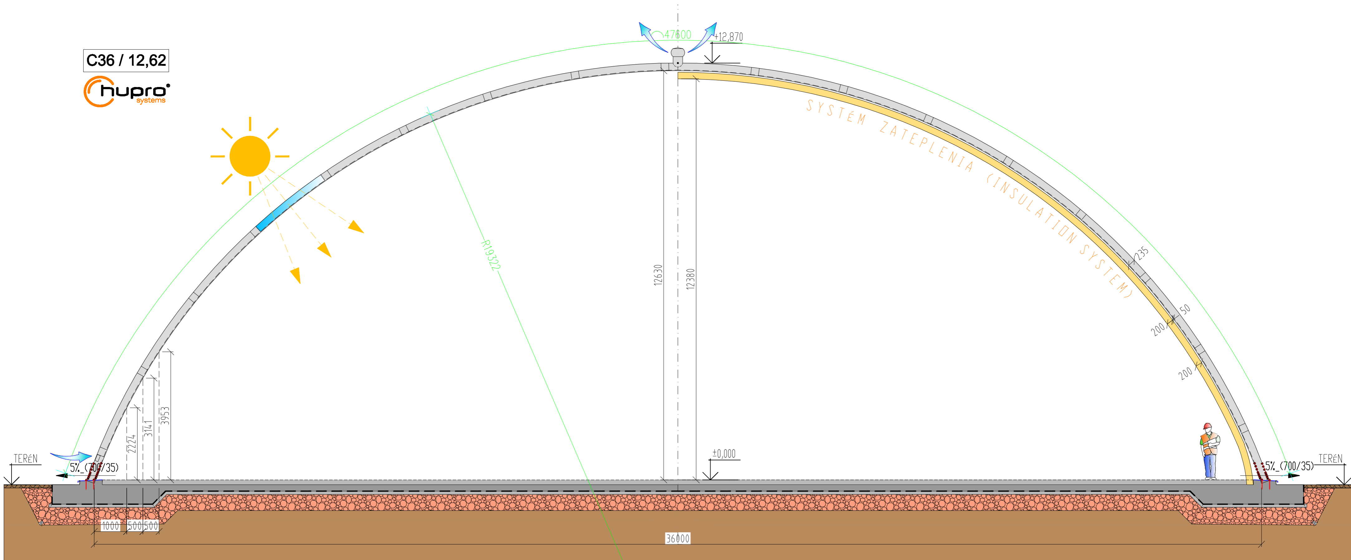
ORIENTAČNÝ TVAR ZAKLADANIA (ORIENTATION FORM OF FOUNDING)
